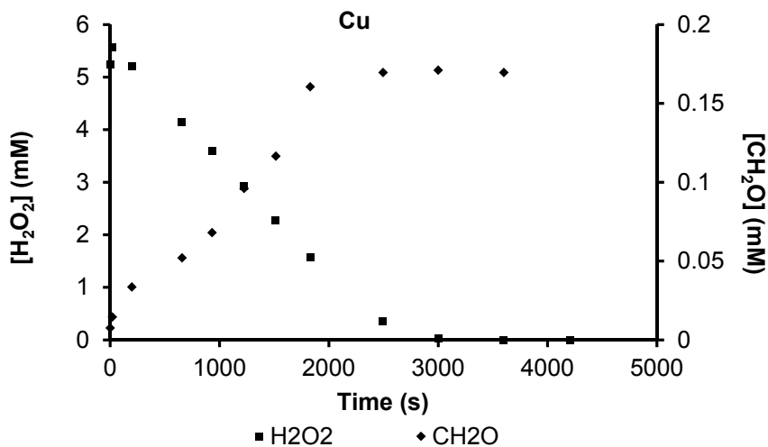
Fig 34. The consumption of H 2 O 2 and the production of CH 2 O as a function of reaction time for Cu-powder. © The Royal Society of Chemistry 2015
