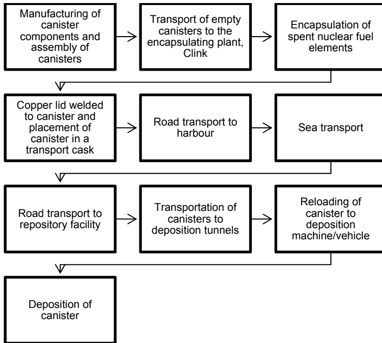
Fig 4. Canister pathway from production to deposition.
