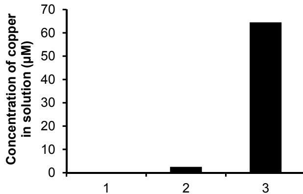
Fig 28. Concentration of copper in solution. 1) Oxidation in air for 96 hours followed by exposure to anoxic pure \text{H}_2\text{O} for 96 hours; 2) \gamma -irradiation in air for 96 hours, 0.1 \text{ Gy}\cdot\text{s}^{-1} , followed by exposure to anoxic pure \text{H}_2\text{O} for 96 hours; 3) \gamma -irradiation in air for 96 hours, 0.14 \text{ Gy}\cdot\text{s}^{-1} , followed by exposure to \gamma -irradiation in anoxic pure \text{H}_2\text{O} for 96 hours, 0.2 \text{ Gy}\cdot\text{s}^{-1} .
