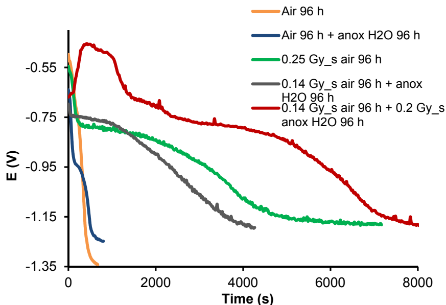
Fig 24. Results from cathodic reduction measurements of polished copper surfaces, irradiated and unirradiated, in humid air.
