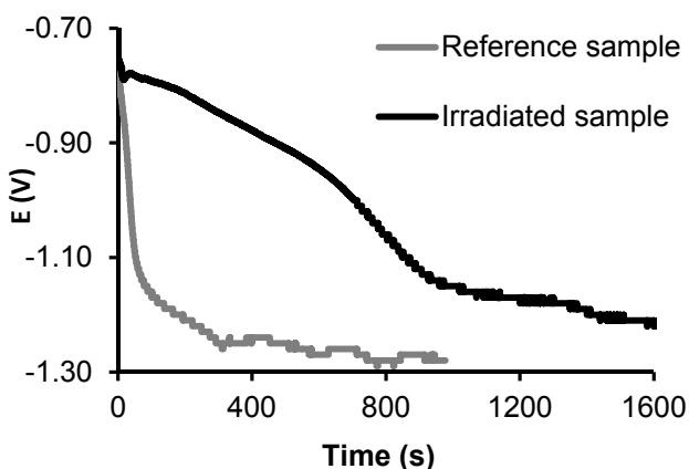
Fig 9. Results from cathodic reduction measurements of an irradiated copper surface and a reference copper surface. © Elsevier B.V.
