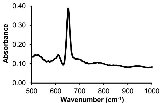
Fig 7. IRAS spectra of an irradiated copper surface. The dose rate was 0.1 Gy·s -1 and the total dose absorbed was 26.7 kGy. © Elsevier B.V.
