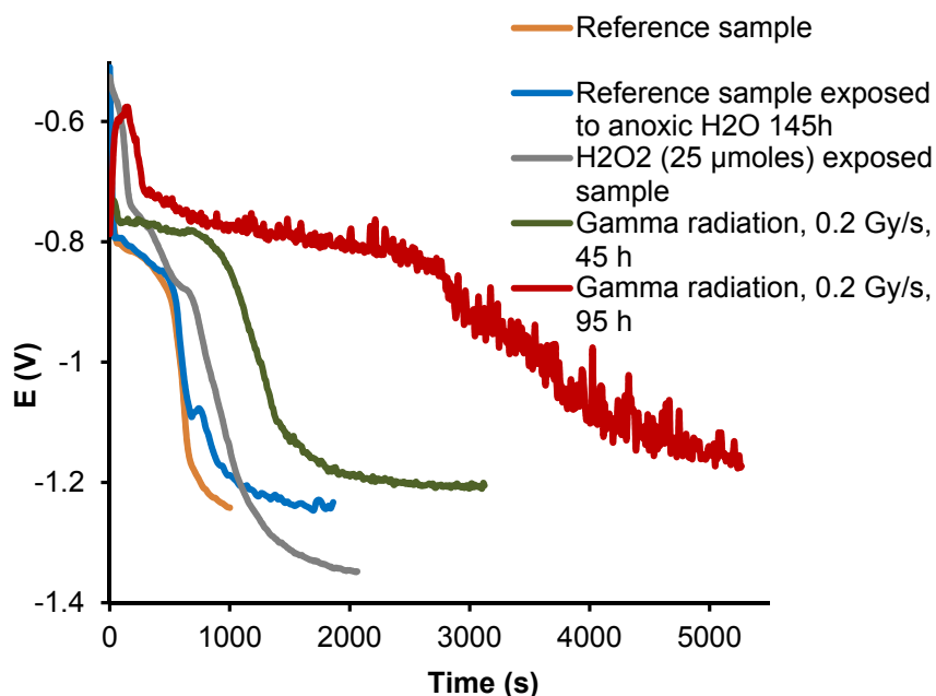
Fig 16. Results from cathodic reduction measurements of irradiated pre-oxidized copper surfaces and reference pre-oxidized copper surfaces.
