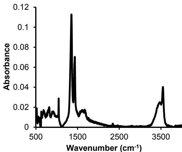
Fig 22. IRAS spectrum of a sample exposed to gamma radiation in air of 60 % RH at a dose rate of 0.14 \text{ Gy}\cdot\text{s}^{-1} for 96 hours.
