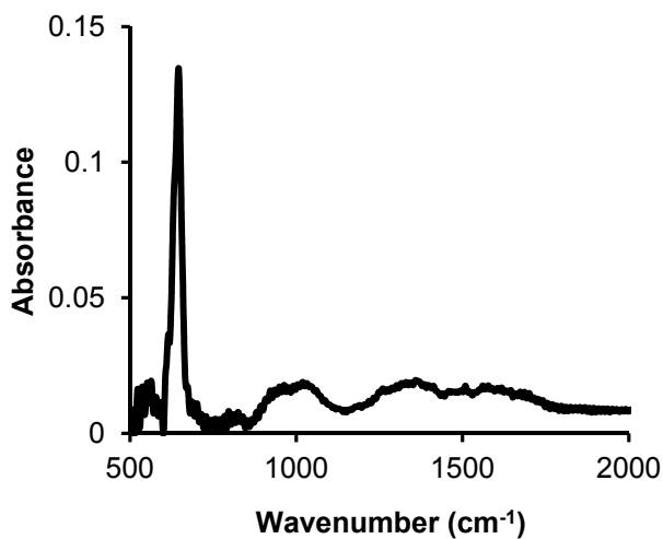
Fig 23. IRAS spectrum of a copper surface irradiated at a dose rate of 0.14 \text{ Gy}\cdot\text{s}^{-1} in air of 60 % RH for 96 hours followed by exposure to anoxic water under gamma radiation at a dose rate of 0.2 \text{ Gy}\cdot\text{s}^{-1} for 96 hours.
