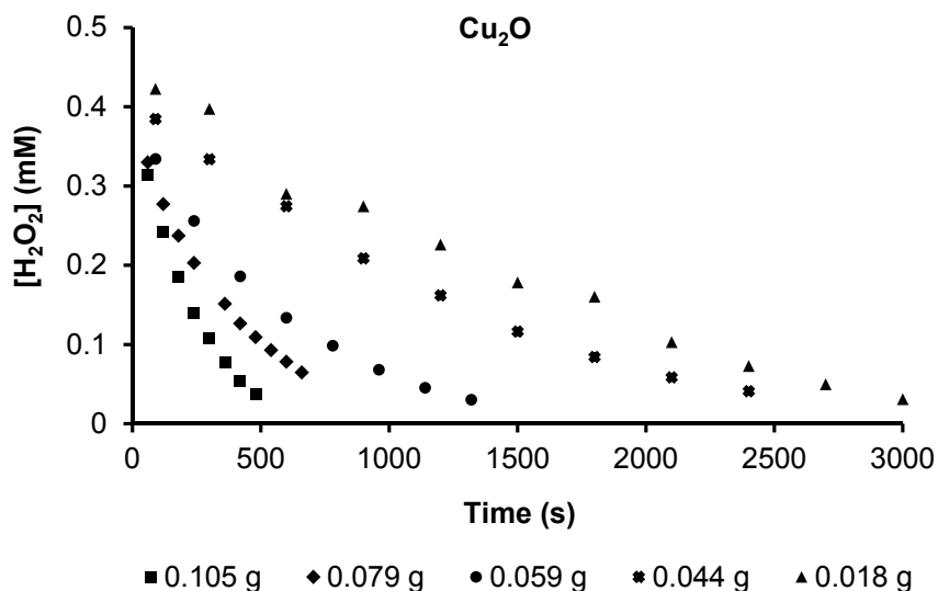
Fig 30. The concentration of H 2 O 2 as a function of reaction time on Cu 2 O-powder. © The Royal Society of Chemistry 2015
