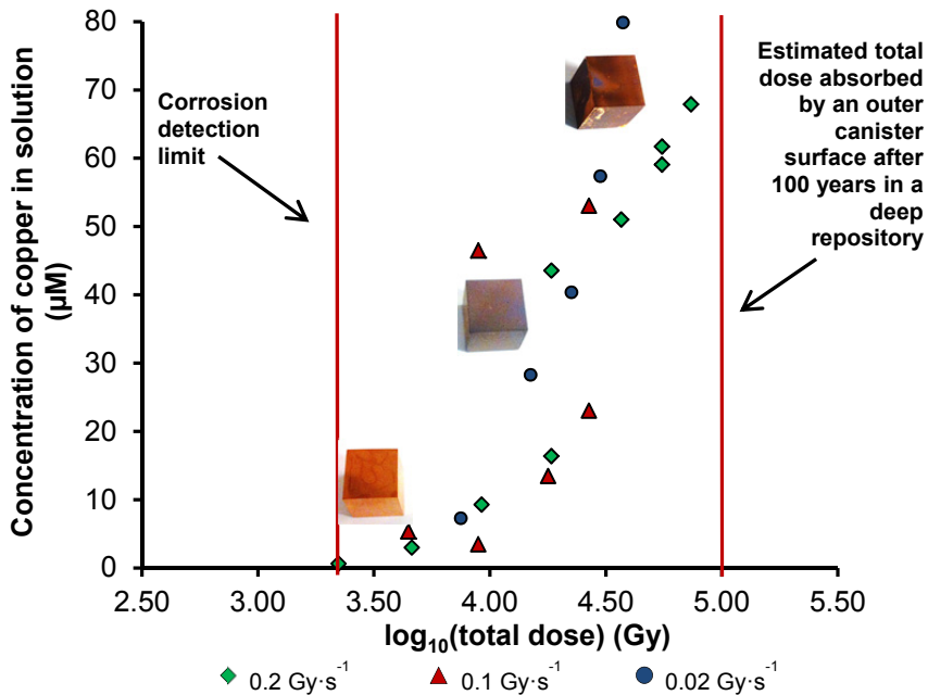
Fig 6. Measured concentrations of copper ( \mu\text{M} ) in aqueous solution as a function of absorbed total dose (Gy). Corrections for the unirradiated reference samples are made. © Elsevier B.V.
