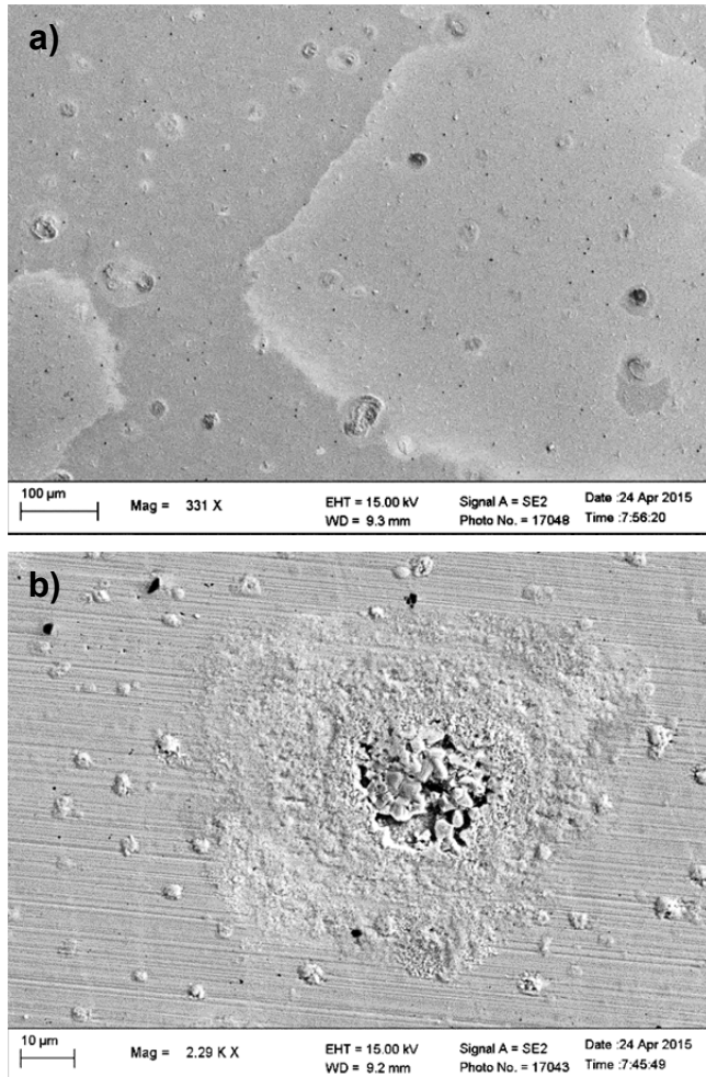
Fig 20 a) and b). SEM images of a polished copper surface irradiated in water-saturated argon at a dose rate of 0.13 \text{ Gy}\cdot\text{s}^{-1} for 96 hours.
