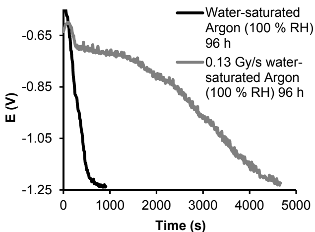
Fig 19. Results from cathodic reduction measurements of polished copper surfaces, irradiated and unirradiated, in water-saturated Argon.
