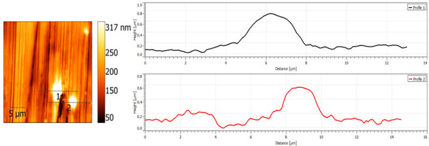
Fig 27. AFM image and surface profiles of particles on a copper surface irradiated at a dose rate of 0.11 \text{ Gy}\cdot\text{s}^{-1} for 96 hours in air of 60 % RH
