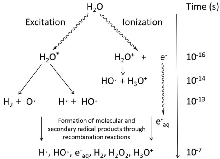
Fig 5. Time scale for the radiolysis of neutral water.
