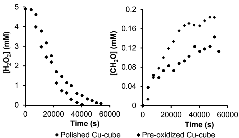
Fig 37. The consumption of \text{H}_2\text{O}_2 and the production of \text{CH}_2\text{O} as a function of reaction time for copper cubes. © The Royal Society of Chemistry 2015
