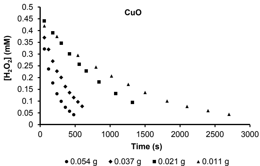
Fig 31. The concentration of H 2 O 2 as a function of reaction time on CuO-powder. © The Royal Society of Chemistry 2015
