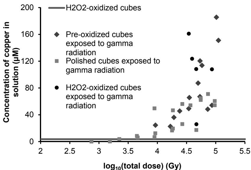
Fig 14. Measured concentrations of copper in solution after irradiations of polished and pre-oxidized copper cubes.
