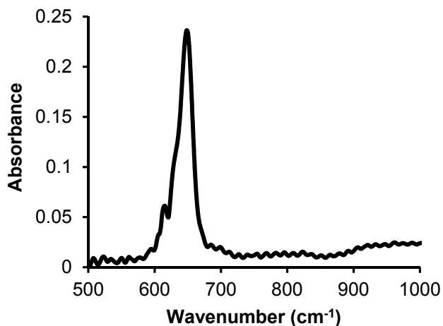
Fig 18. IRAS spectrum of a sample exposed to gamma radiation in water-saturated Argon at a dose rate of 0.13 \text{ Gy}\cdot\text{s}^{-1} for 96 hours.
