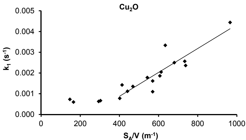
Fig 33. An enlargement of the first-order rate constants k_1 ( s^{-1} ) for consumption of H_2O_2 on Cu_2O -powder plotted against solid surface-area-to-solution-volume ratios. © The Royal Society of Chemistry 2015
