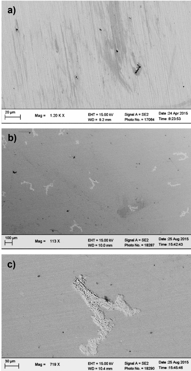
Fig 17 a, b and c. SEM-images of a reference pre-oxidized copper (a) and irradiated pre-oxidized copper (b and c).
