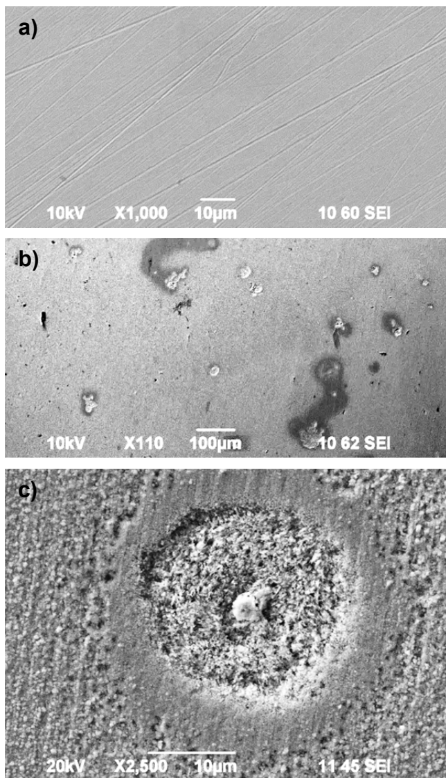
Fig 10 a, b and c. SEM-images of a) a reference copper surface exposed to anoxic pure water for 96 hours , b) an irradiated copper surface using a dose rate of 0.1 \text{ Gy}\cdot\text{s}^{-1} and a total dose of 62 kGy and c) a close-up on one of the local corrosion features.
