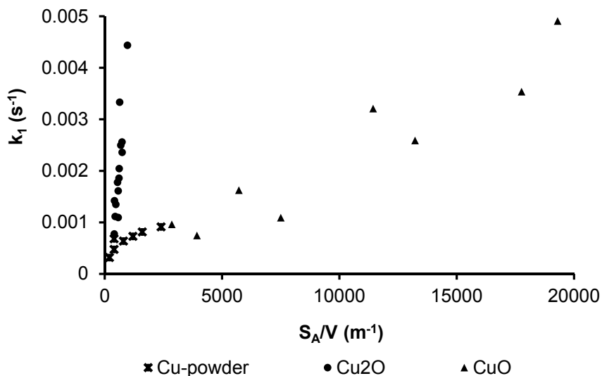
Fig 32. First-order rate constants ( k_1 ( \text{s}^{-1} )) as a function of solid surface-area-to-solution-volume ratios. © The Royal Society of Chemistry 2015
