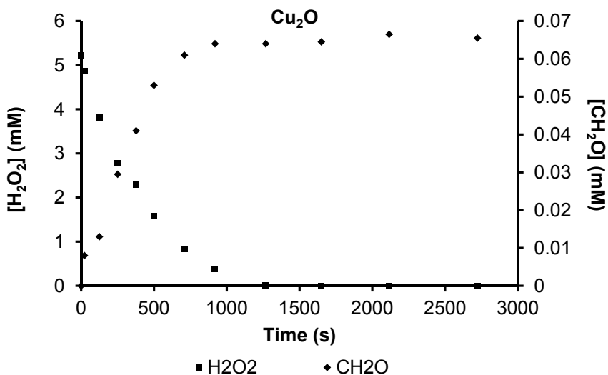
Fig 35. The consumption of H 2 O 2 and the production of CH 2 O as a function of reaction time for Cu 2 O-powder. © The Royal Society of Chemistry 2015
