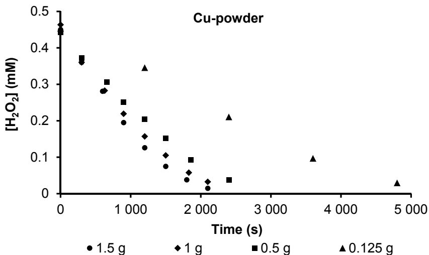
Fig 29. The concentration of \text{H}_2\text{O}_2 as a function of reaction time on Cu-powder. © The Royal Society of Chemistry 2015
