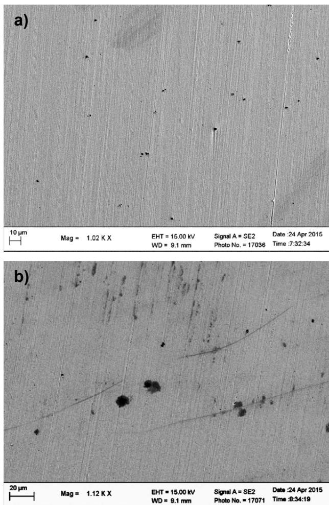
Fig 25 a) and b). SEM images of a) a copper surface irradiated at a dose rate of 0.25 \text{ Gy}\cdot\text{s}^{-1} for 96 hours in air and b) a copper surface irradiated in air at followed by exposure to anoxic water.
