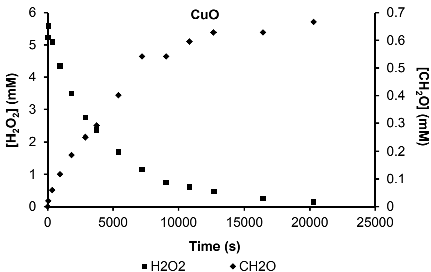
Fig 36. The consumption of H 2 O 2 and the production of CH 2 O as a function of reaction time for CuO-powder. © The Royal Society of Chemistry 2015
