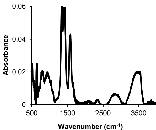
Fig 21. IRAS spectrum of a copper surface irradiated at a dose rate of 0.13 \text{ Gy}\cdot\text{s}^{-1} in air of 100 % RH for 96 hours.
