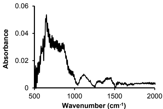
Fig 15. IRAS spectrum of a pre-oxidized copper cube (90°C dry air for 24 hours) exposed to gamma radiation using a dose rate of 0.25 \text{Gy}\cdot\text{s}^{-1} for 96 hours.
